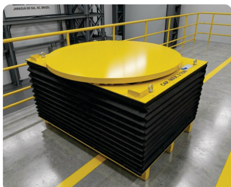
MESA MOLA
